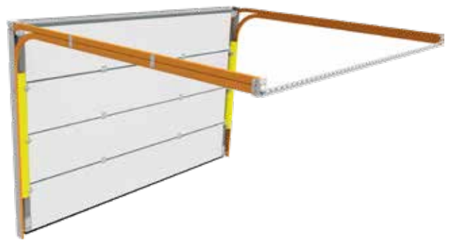
Track Z – minimum lintel height of 80 mm (manual) or 120 mm (automatic)
