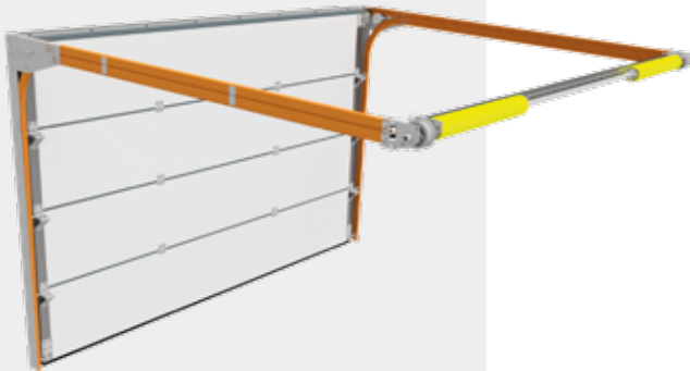
Track R – minimum lintel height of 80 mm (manual) or 120 mm (automatic)
