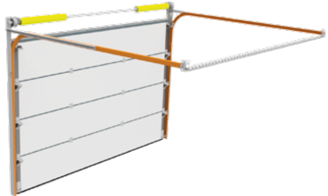
Track S – minimum lintel height of 350 mm
