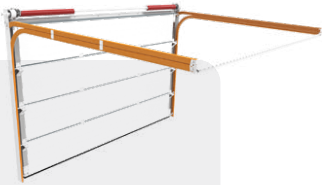
Track F – minimum lintel height of 200 mm
